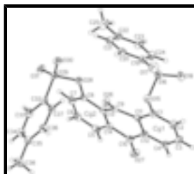
Fig. 1. The molecular structure of the title compound showing the atom-labeling scheme. Displacement ellipsoids are drawn at the 25% probability level, and H atoms are shown as small spheres of arbitrary radius. Cg1 and Cg2 are the centroids of the C1—C4/C11/C12 and C5—C8/C13/C14 rings respectively.
