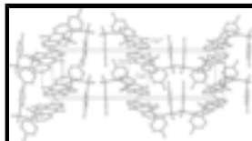
Fig. 3. The arrangement of the molecules in the crystal structure viewed approximately along c axis. The C—O... \pi interactions are represented by dotted lines. H atoms not involved in interactions have been omitted. [Symmetry codes: (iv) -x, -y + 1, -z + 1 ; (v) -x + 1, -y + 1, -z + 1 .]
